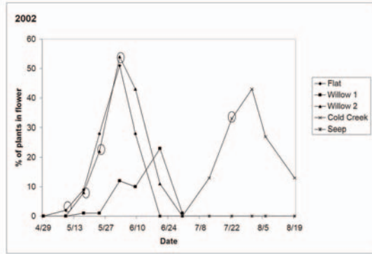
FIG. 2a. Phenology of Eriogonum umbellatum near Willow Creek, Spring Mountains, Nevada during 2002 (encircled data-points indicate presence of adult Euphilotes ; see text for locations of transects).
